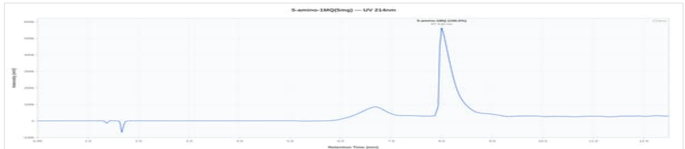
5-Amino-1MQ 5mg - VRL-9485675: UV Chromatogram
