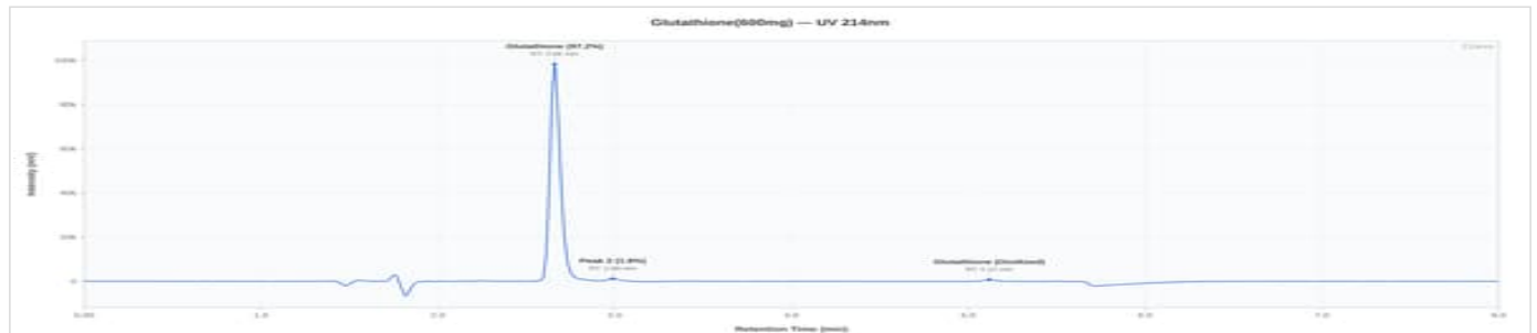
Glutathione 600mg - VRL-8350331: UV Chromatogram
