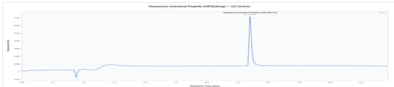
VIP 10mg - VRL-8713624: UV Chromatogram
